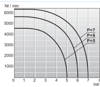
Flow diagram 1/2"
