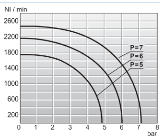
Flow diagram 1/4"
