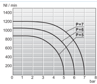
Flow diagram 1/8"
