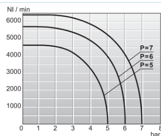
Diagram pretoka 1/2"
