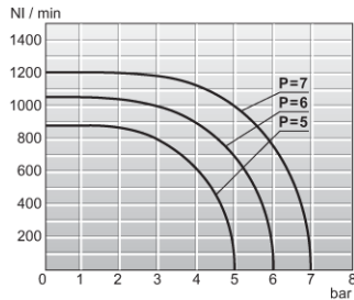
Flow diagram 1/8"
