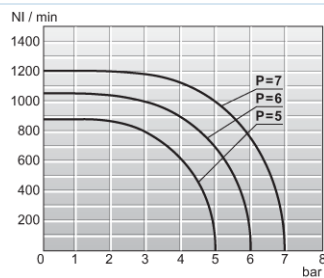
Dijagram protoka 1/8"
