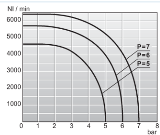
Dijagram protoka 1/2"
