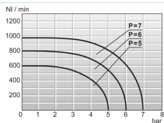
Diagram pretoka 1/8"
