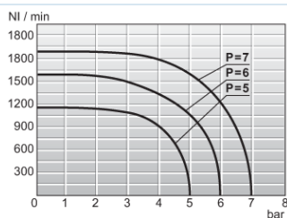
Diagram pretoka 1/4"
