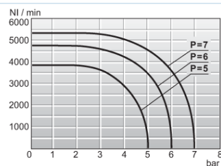
Diagram pretoka 1/2"
