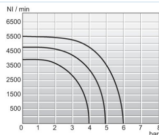
Dijagram protoka 1/2"
