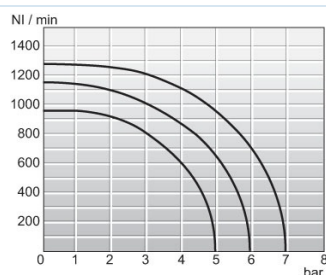
Diagram pretoka 1/8"
