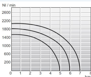
Diagram pretoka 1/4"
