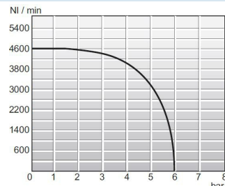
Diagram pretoka 1/2"
