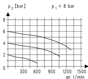
Diagram pretoka
