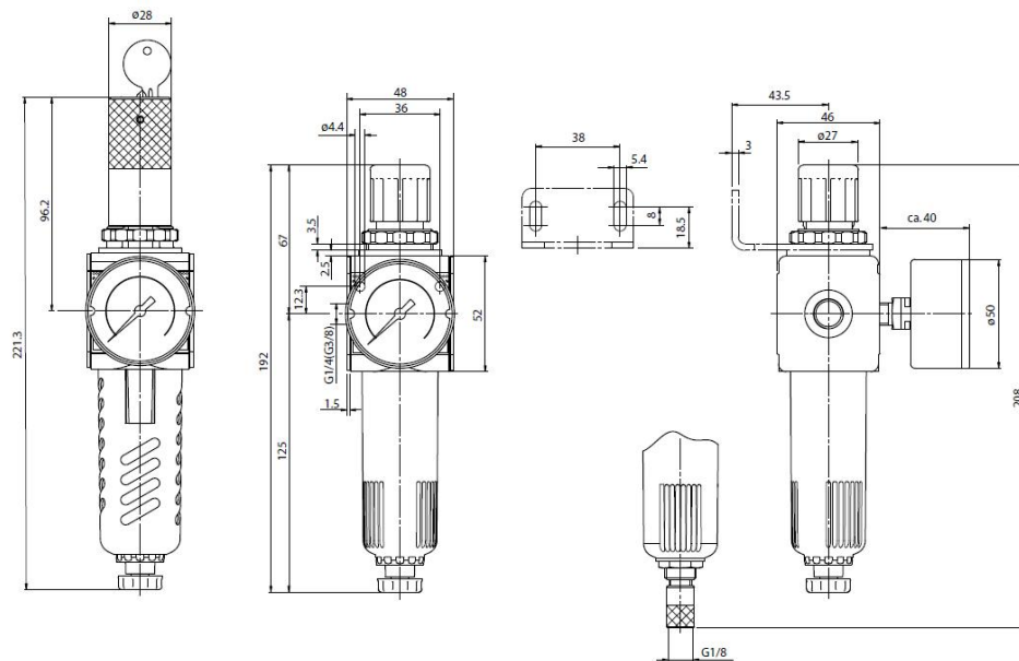
semi-automatic drain valve
