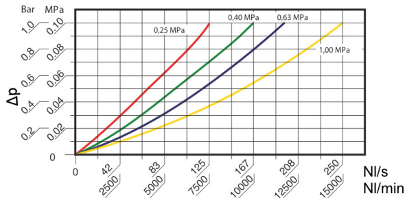
The diagram shows various inlet pressures up to max. 1bar pressure drop
