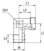
Main body
