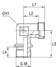
screw fitting
