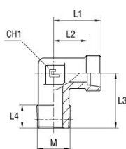
screw fitting
