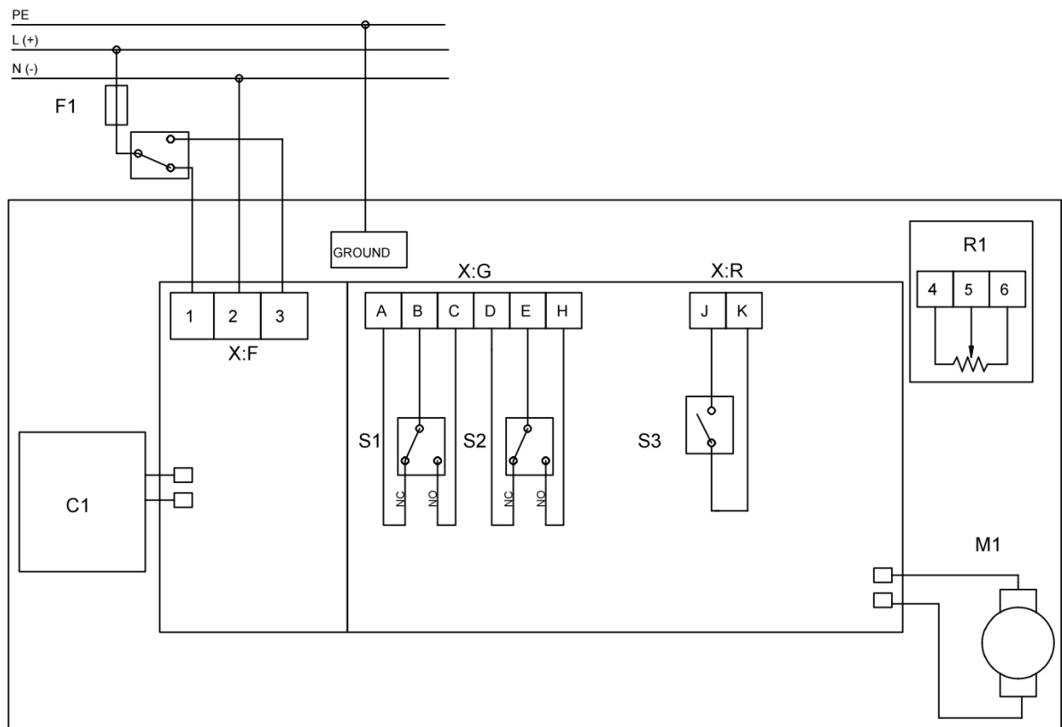
3-point control
