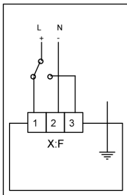
3-point control
