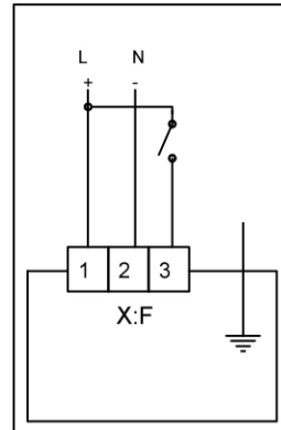
2-point control
