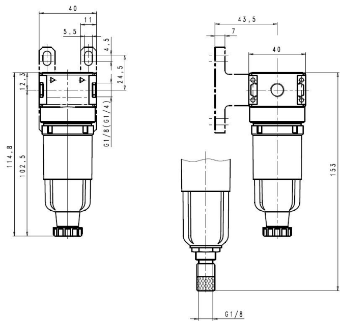
automatic drain valve
