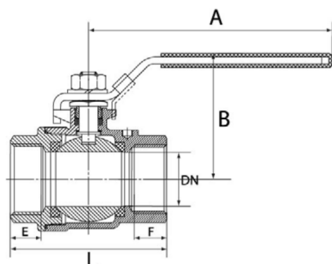
Stainless steel ball valve, 2-piece, female/female thread, with full bore
