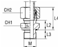
with B4 cutting ring
