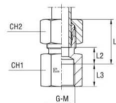
with B3 cutting ring
