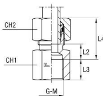
with B4 cutting ring
