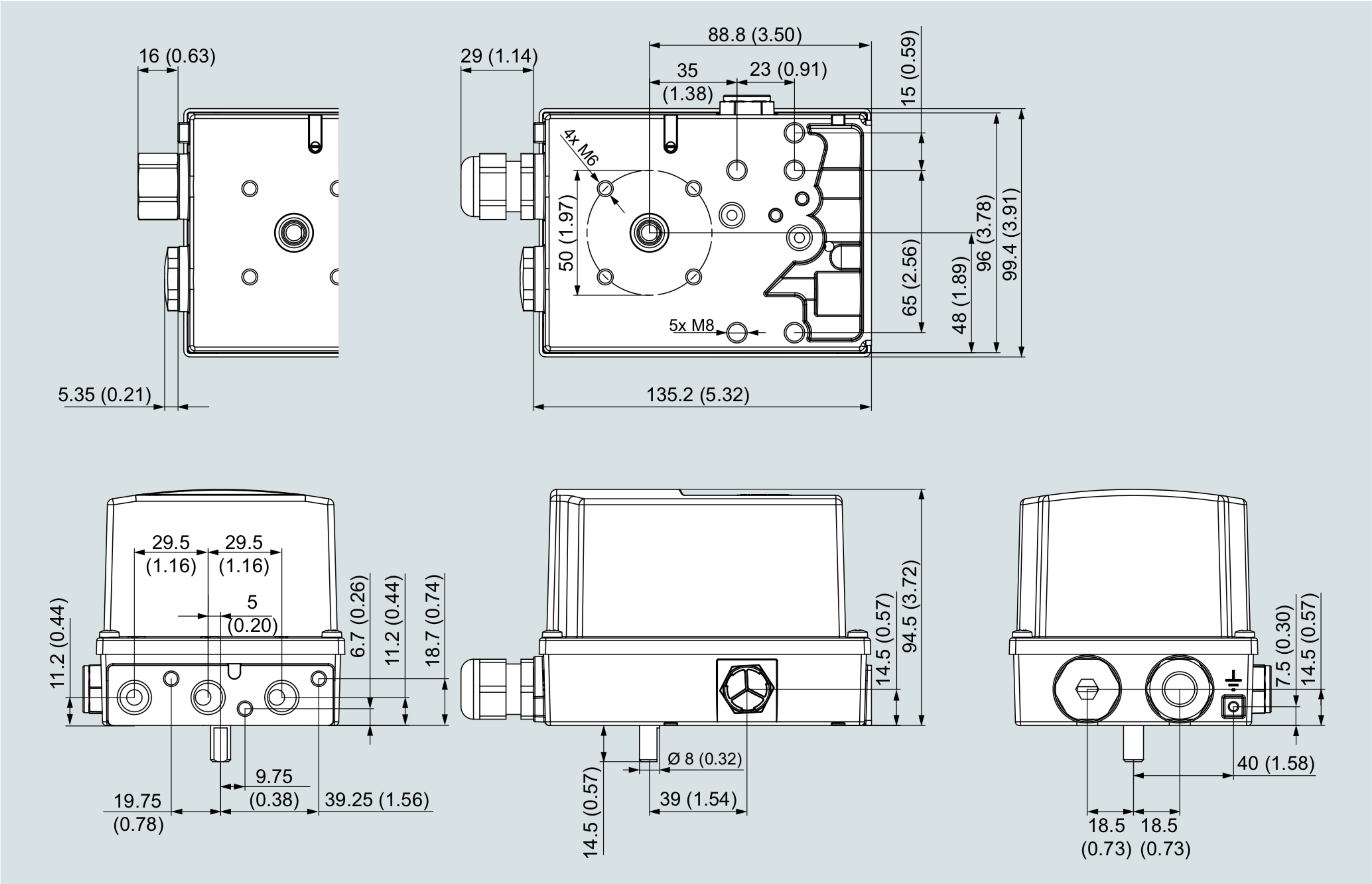
Non-flameproof enclosure, dimensions in mm (inch)
