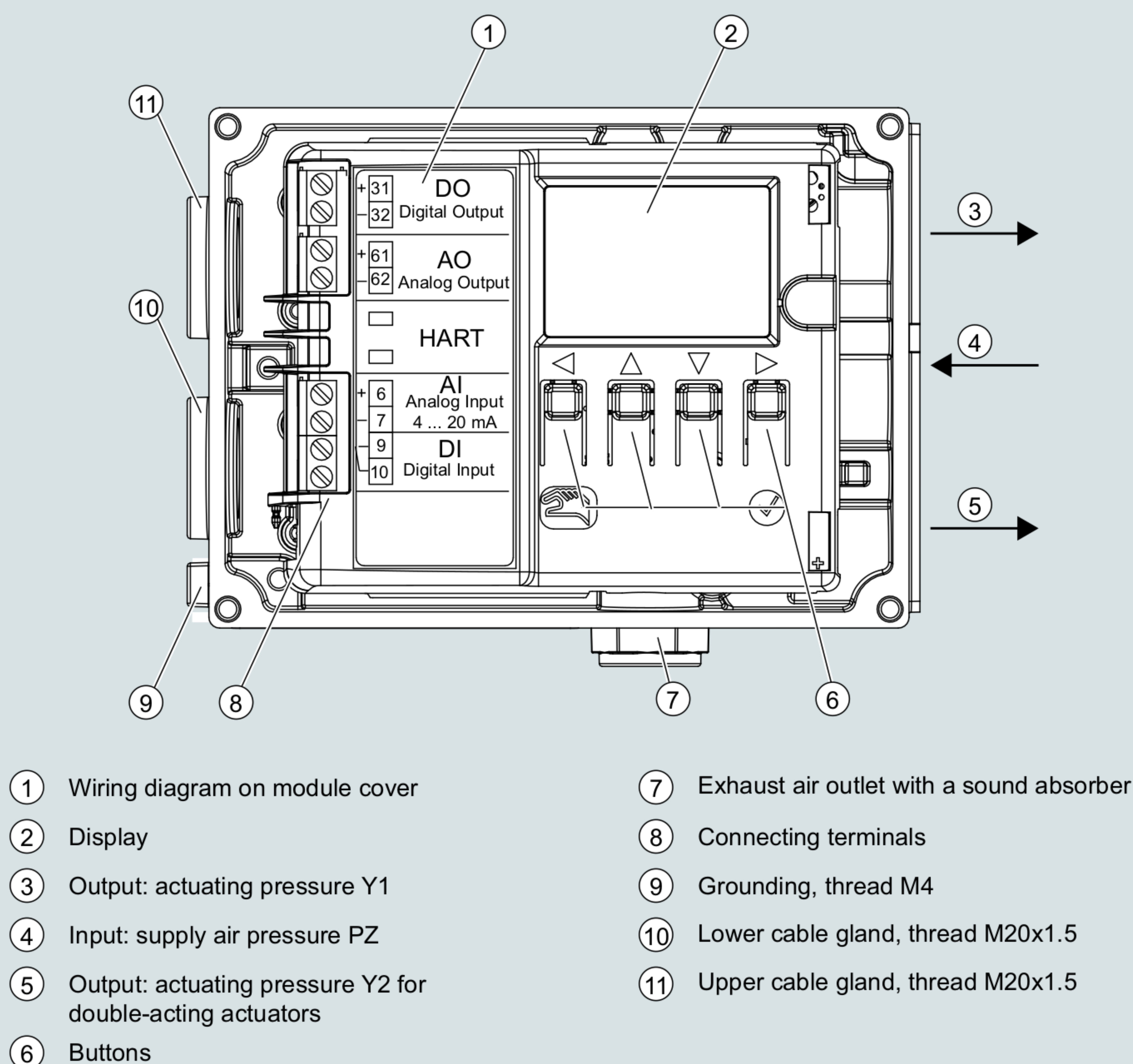
SIPART PS100, enclosure with open lid
