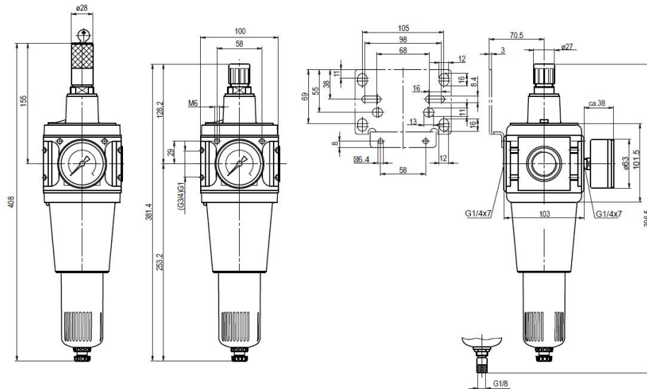
semi-automatic drain valve
