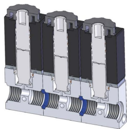
Installation of the O-rings
