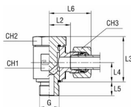
with B4 cutting ring
