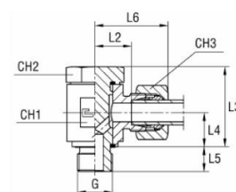
with B3 cutting ring
