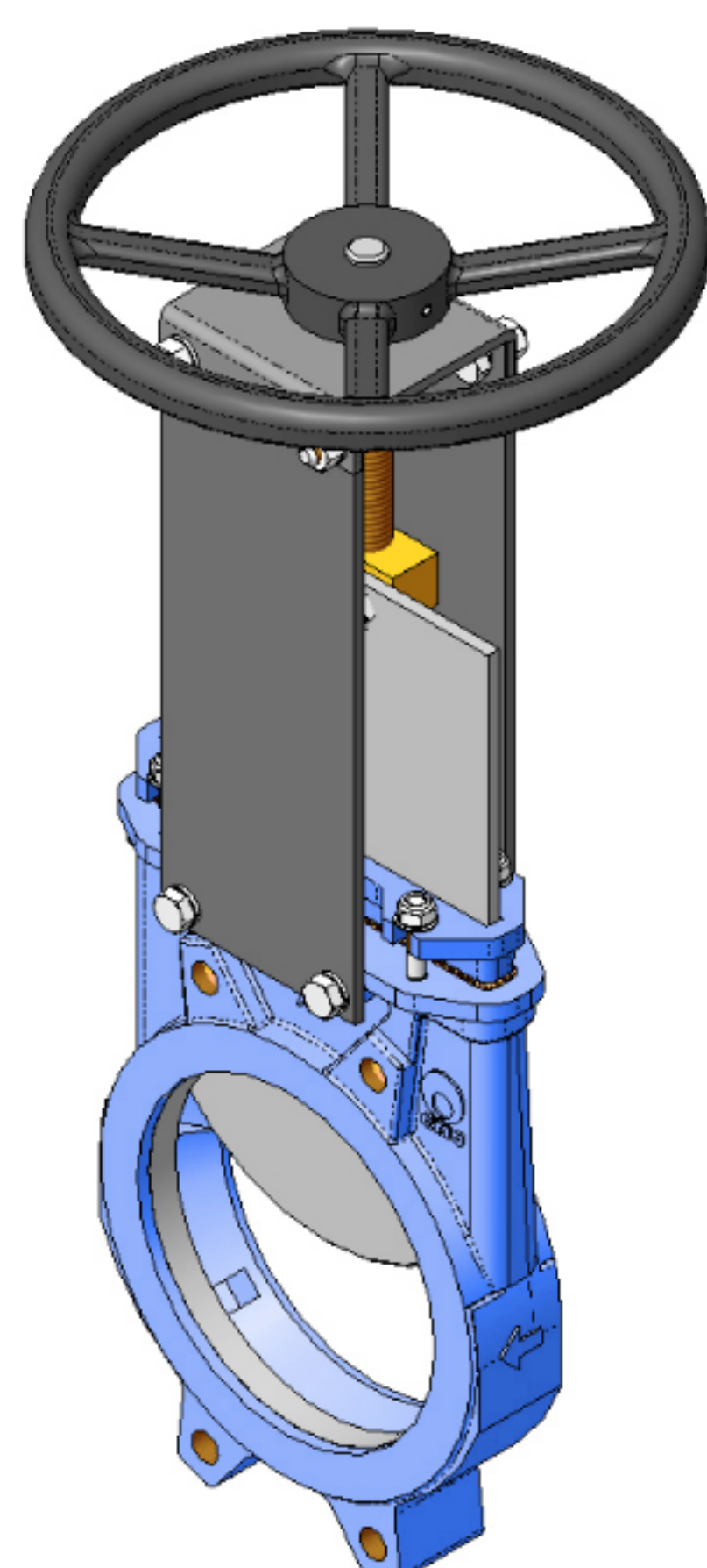
HANDWHEEL NON-RISING STEM
