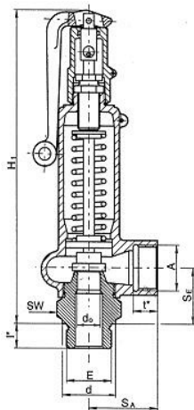
Head Vent lever gas-tight
