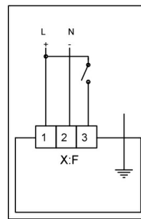
2-point control
