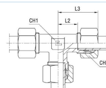
with B3 cutting ring
