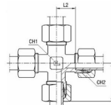
with B3 cutting ring
