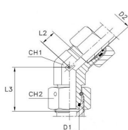
with B4 cutting ring
