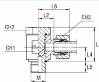
with B4 cutting ring
