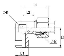
with B4 cutting ring
