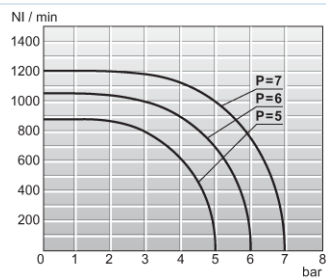
Flowdiagram 1/8"
