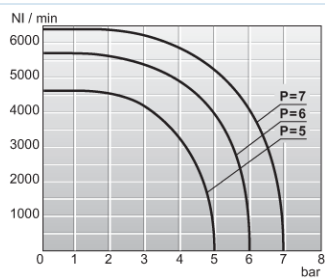
Flowdiagram 1/2"
