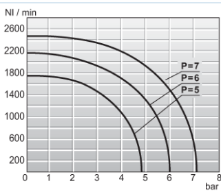
Flowdiagram 1/4"
