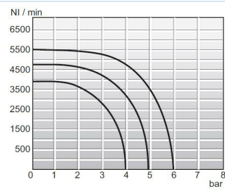
Flowdiagram 1/2"
