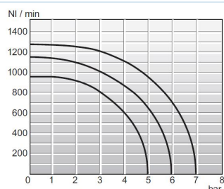
Doorstroombiagramma 1/8"
