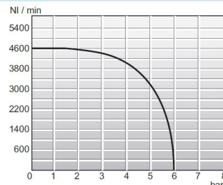
Flowdiagram 1/2"
