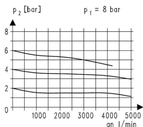
Flowdiagram
