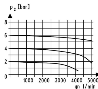
G1/2"
