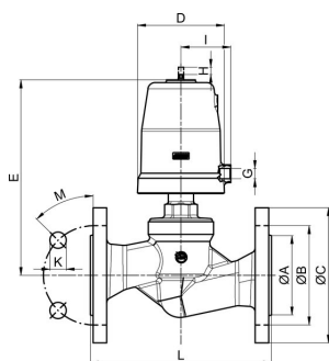
Ressort ferme, Type SE24, SE25, SE33
