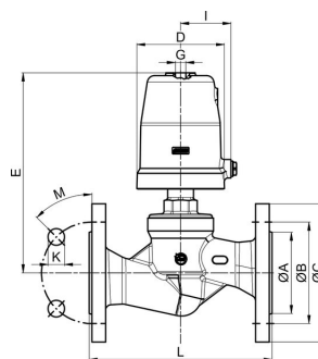
Ressort ouvre, Type SE23
