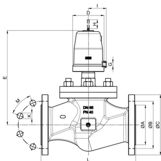
Ressort ferme, Type SE24, SE25, SE33
