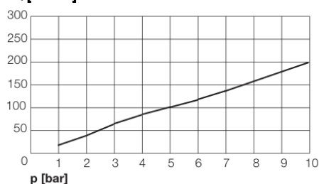
Q [l/min]
