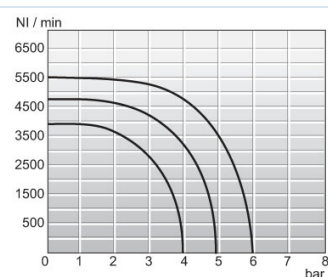
Diagram pretoka 1/2"
