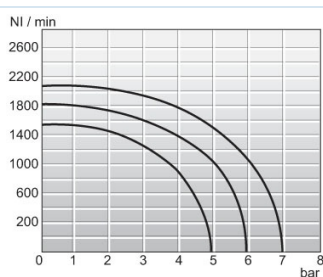
Diagram pretoka 1/4"
